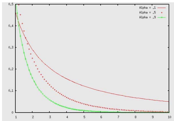
Figure 3: Sample decay curves for various alpha
