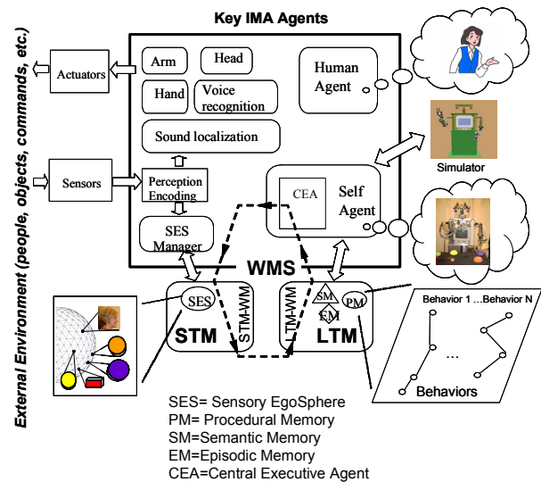
Figure 1: ISAC's Cognitive Robot Architecture
