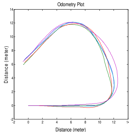
Figure 3: Robot trajectories of the five teleoperation trials according to the odometer.
