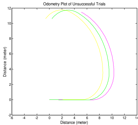
Figure 9: Trajectory plot of the 3 failed evaluation trials according to the odometer. Note that all the failures happened at Boundary 3.
