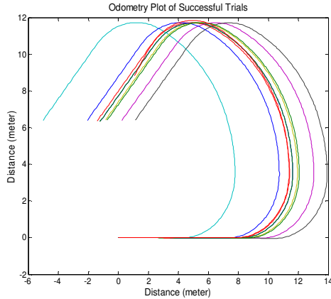
Figure 8: Trajectory plot of the 12 successful evaluation trials according to the odometer. Note that the odometer was reset at the beginning of every trial, and the robot started at different locations for each trial.
